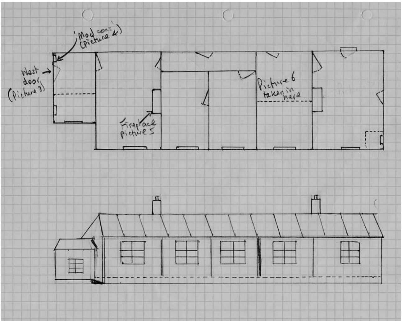
Tin Houses - Front Elevation and Plan
